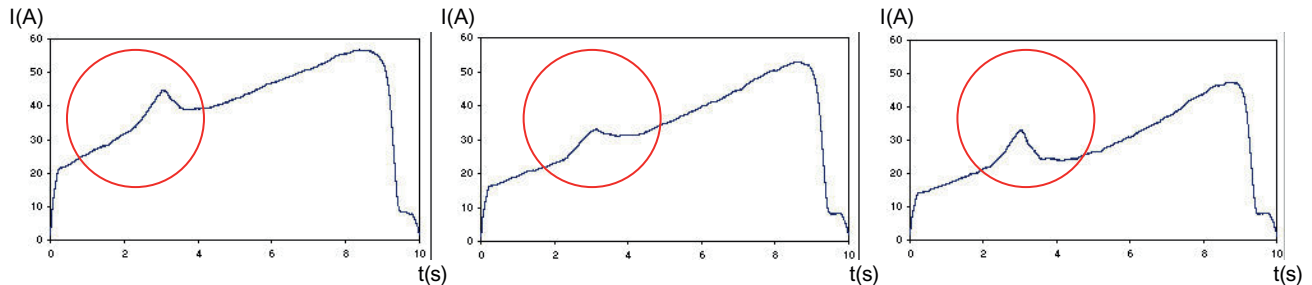
Figure 3-6 Current characteristic and occurrence of DC components in the three phases without "polarity balancing"
