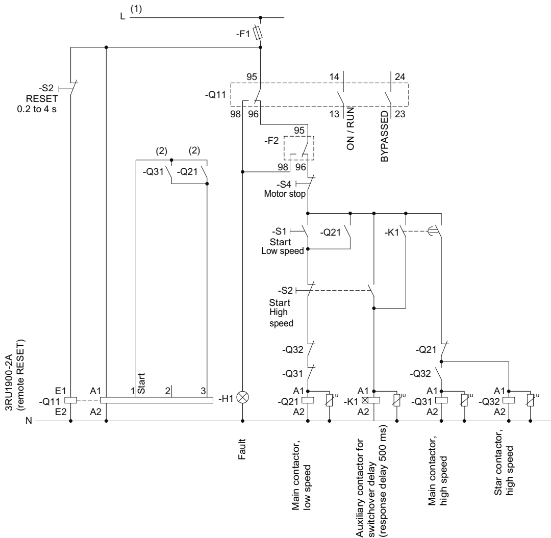
Figure 15-34 Wiring of the 3RW40 5 to 3RW40 7 control circuit
