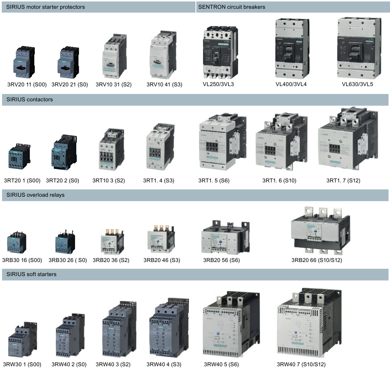
Figure 4-1 SIRIUS modular system
