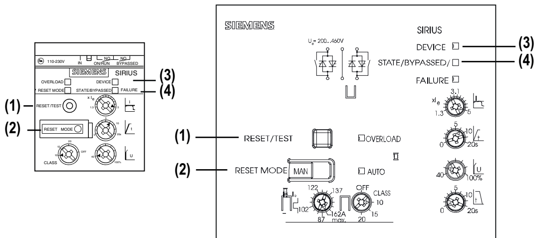
Figure 12-1 Overview of buttons / LEDs on the 3RW40 2 to 3RW40 4 and 3RW40 5 to 3RW40 7
