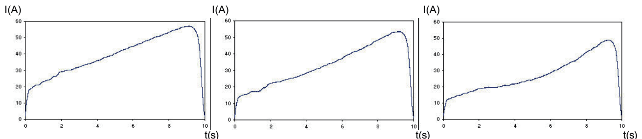
Figure 3-7 Current characteristic in the three phases without DC components thanks to "polarity balancing"
