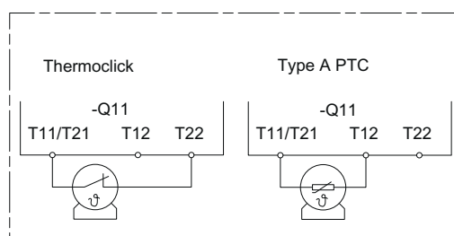
Figure 15-1 Optional thermistor motor protection evaluation
