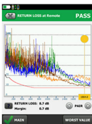
Return loss graph
